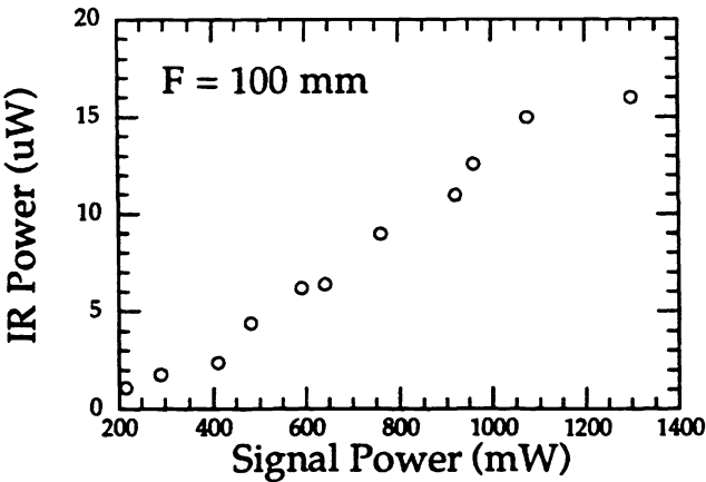
Figure 4. IR power generated as a function of the signal laser power for the case of F = 100 mm. The pump laser power was fixed at 110 mW.
