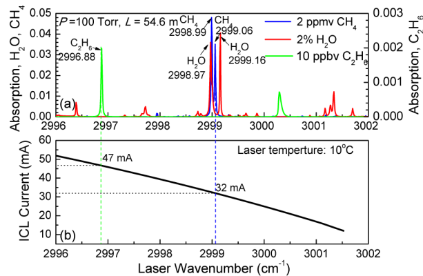
Fig. 2. (a) HITRAN based absorption spectra of \text{C}_2\text{H}_6 (10 ppbv), \text{CH}_4 (2 ppmv), and \text{H}_2\text{O} (2%) in a narrow spectral range from 2996\text{ cm}^{-1} to 3002\text{ cm}^{-1} at a pressure of 100 Torr and an absorption length of 54.6 m. \text{C}_2\text{H}_6 , \text{CH}_4 , and \text{H}_2\text{O} lines are shown in green, blue and red, respectively. (b) Plot of the ICL emission wavenumber as a function of the ICL drive current at 10^\circ\text{C} .
