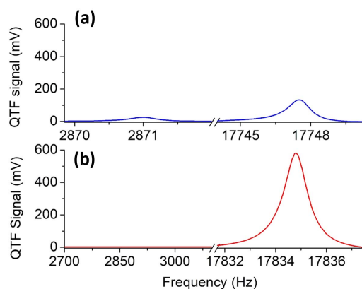
Fig. 4. Resonance curves measured at a fixed excitation level V = 300 mV and at atmospheric pressure for the (a) QTF-Q and (b) QTF-O.
