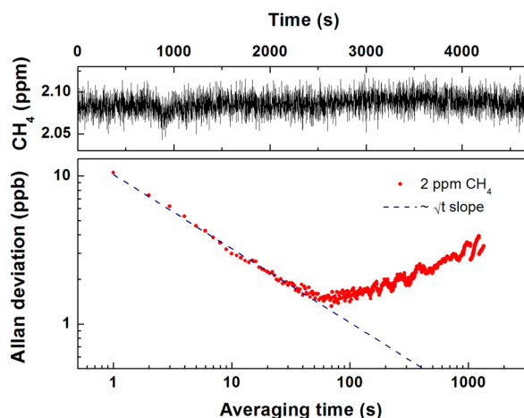
FIG. 3. Allan-Werle deviation plot acquired from measurements using a certified 2 ppm CH 4 cylinder with a 1 Hz sampling rate.
